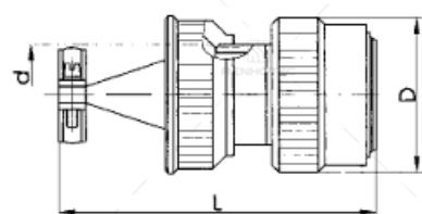
8 - Plug with angled clamp cable tail attachment
