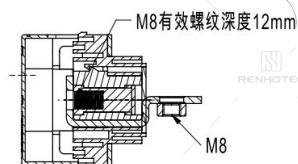
SECTION H-H
