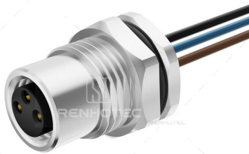
M8 Female Panel Mount Cable Assembly, Front Fastened, Unshielded, Straight
