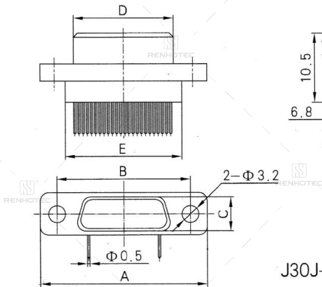
J30J-9~100TJW-J
