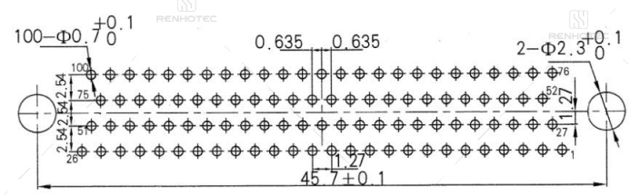
J30J-100TJN-J
