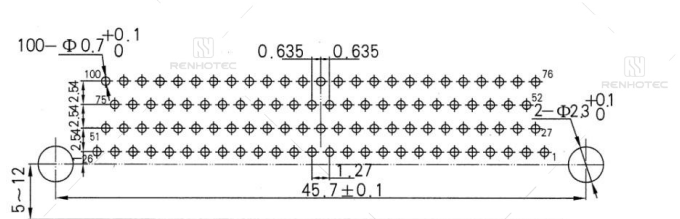
J30J-100TJW-J
