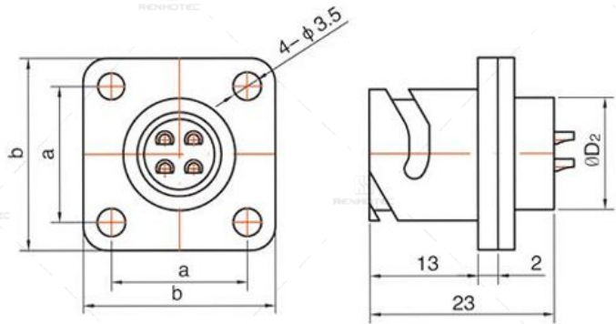
方盘插座: Square Flange Receptacle
