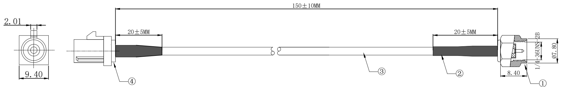
Fakra Plug C Code Blue
