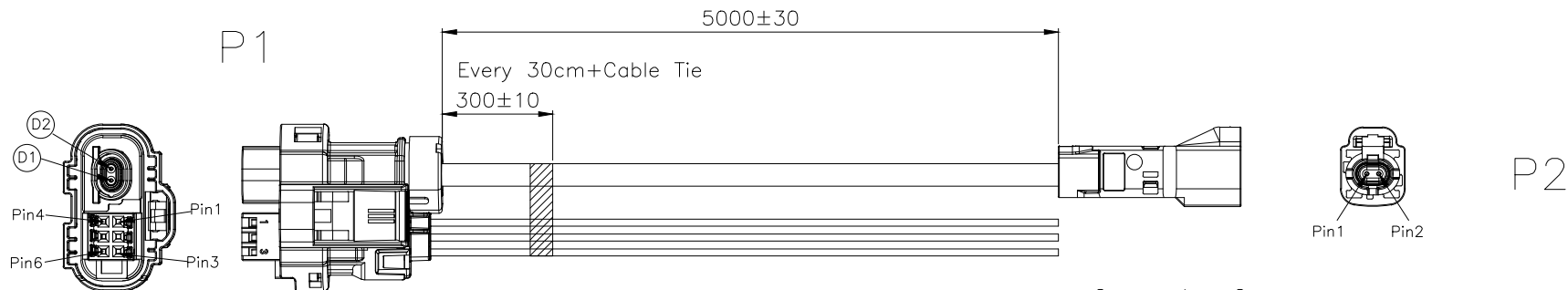
Connector 2: Rosenberger : E6S10A-1CAZ5-Z
