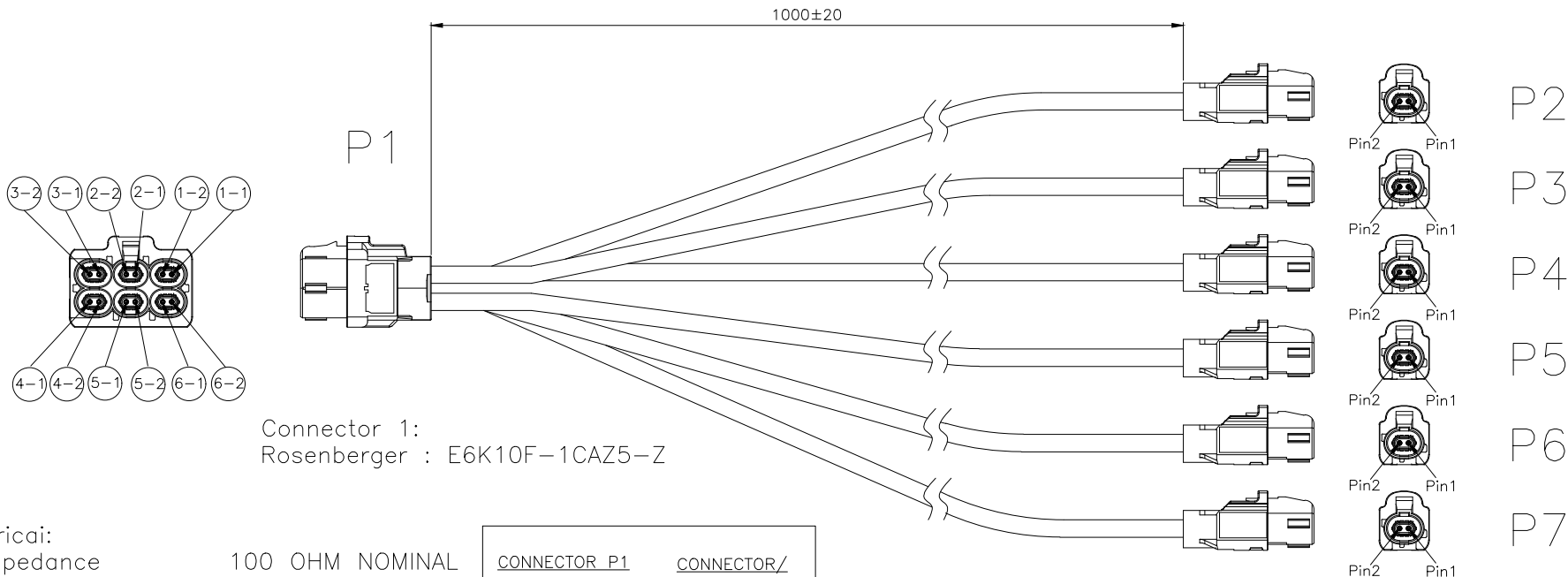
Connector 2/3/4/5/6/7: Rosenberger : E6K10A-1CAZ5-Z
