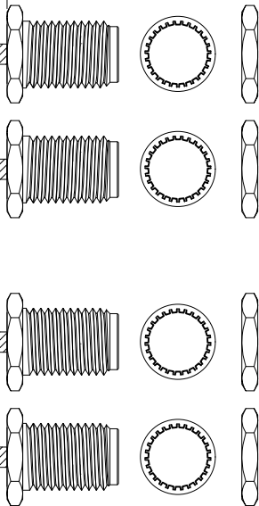
CONNECTOE 2/3/4/5: SMA FEMALE
