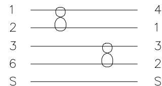
CONNECTOR P1 CONNECTOR P2
