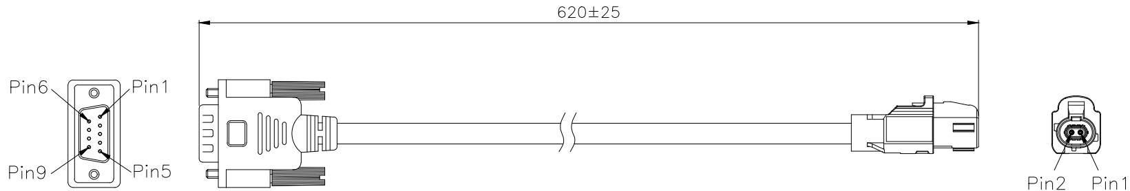
Connector 2: Rosenberger : E6K10A-1CAZ5-Z
