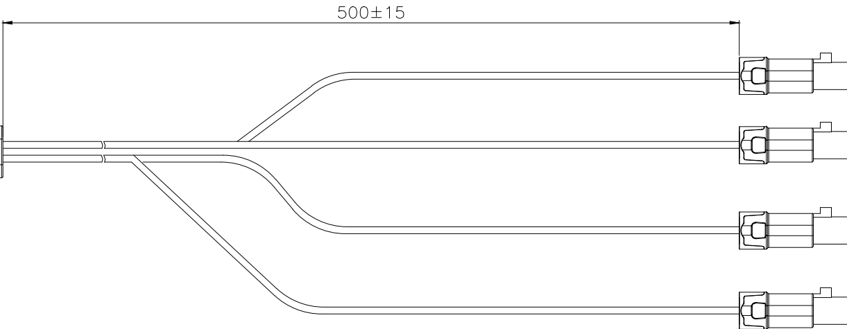
Connector 2/3/4/5: TE : 2-2307198-0
