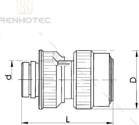
13 - Plug with type 09 thermoplastic sleeve tail attachment
