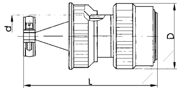
8 - Plug with angled clamp cable tail attachment
