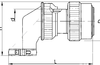
8 - Plug with angled clamp cable tail attachment
