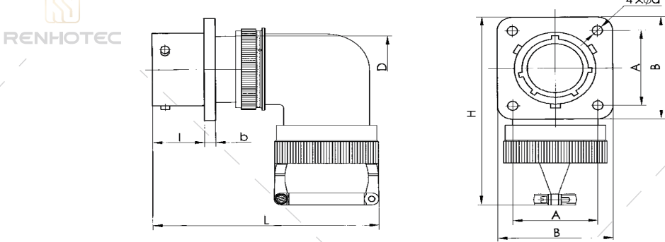
27 - Socket with type 11 shielded elbow cable tail attachment
