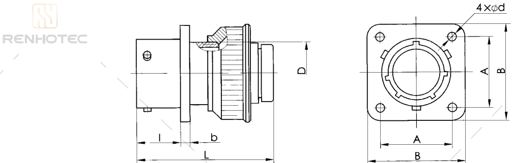
12 - Socket with type 09 thermoplastic sleeve type tail attachment
