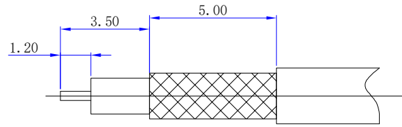
Recommended stripping size
