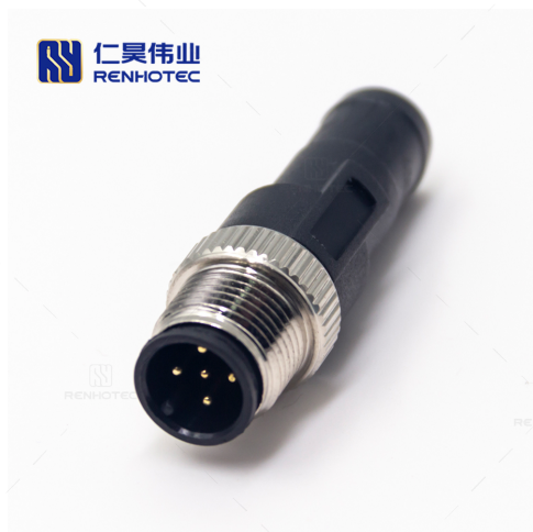
M12 Male Plug Straight Plastic Shell Terminator Field Wireable Connector, IP67 Rugged Connector
