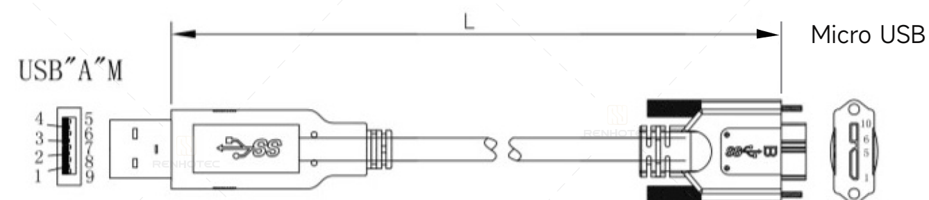
USB3.0 Diagram
