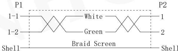
*Wiring Table
