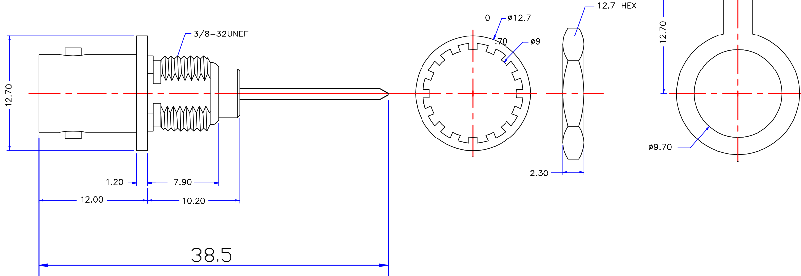
RECOMMENDED MOUNTING HOLE
